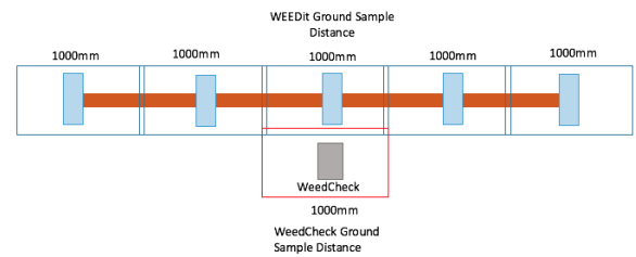
Figure 3.11: WeedCheck installation on WEEDit Boom
