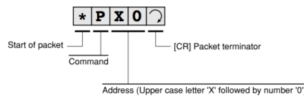
Figure 4.4: WEEDit Poll Request
